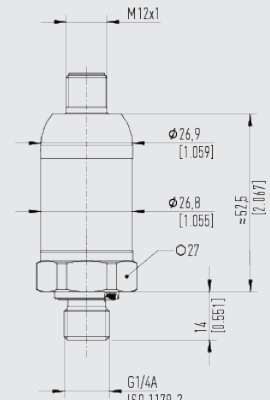
With circular connector M12 x 1 (4-pin, metallic)
