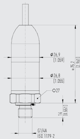
With cable outlet IP68, FEP, IP6K9K
